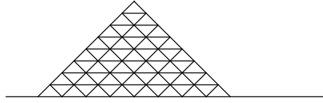
Figure 4: h_{\alpha,2^{-k}} = \sum_{i=1}^{2^{2p}} h_{\beta_i,2^{-p-k}} . Here, p = 3 .
