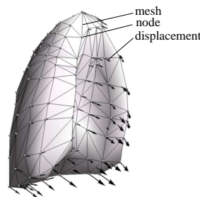
Figure 1: FEM result: node displacements
