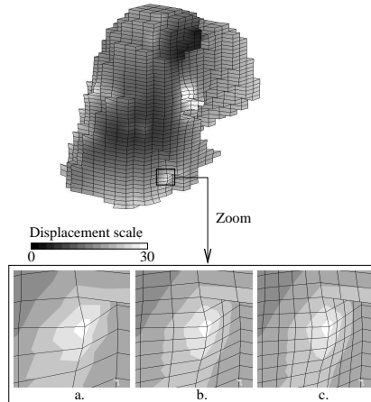
Figure 3: Mesh subdivision. Subdivision number for zoomed details: a. : 1 - b. : 2 - c. : 4
