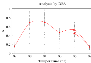
Figure 6: Detrended fluctuation analysis. \alpha vs. temperature. Black points are \alpha values, red ones are main median vales of \alpha at corresponding temperature
