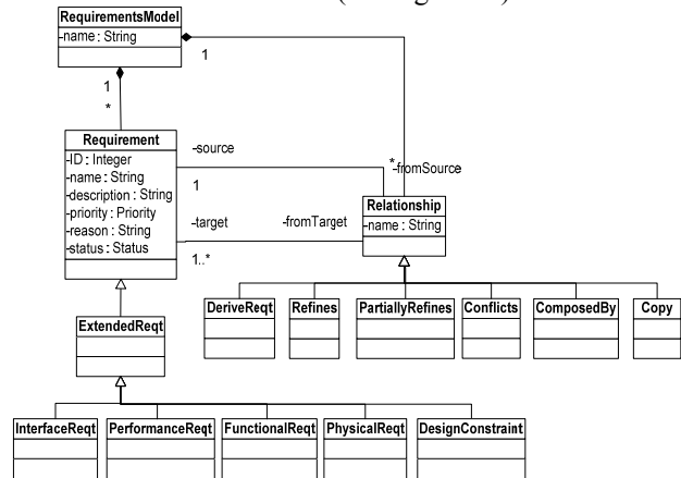
Figure 10 Specialized Requirements Metamodel for SysML Requirements
