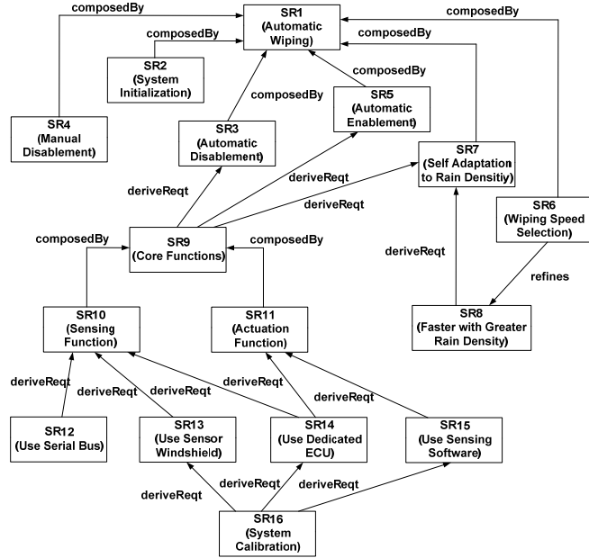
Figure 11 SysML Model for the Rain Sensing Wiper System [14]
