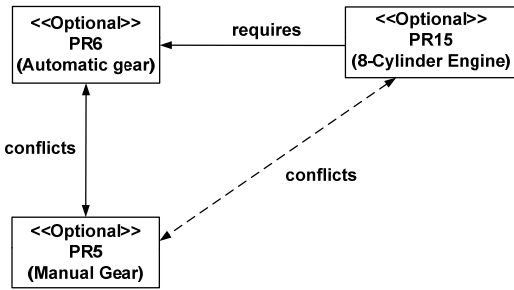
Figure 8 Example Inferred Conflicts Relation
