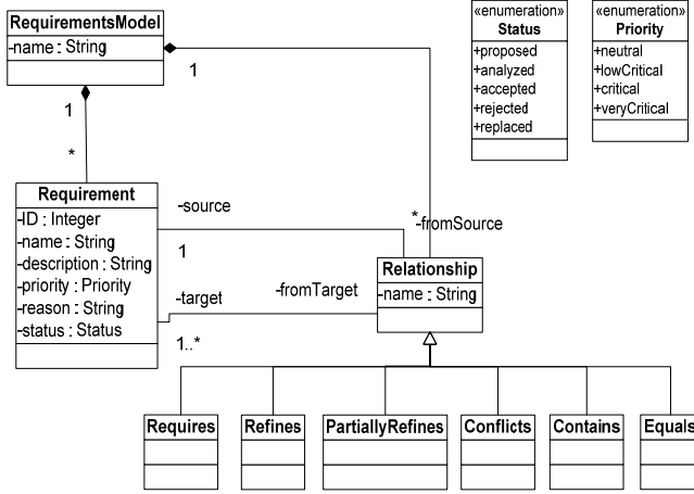
Figure 2 Core Requirements Metamodel
