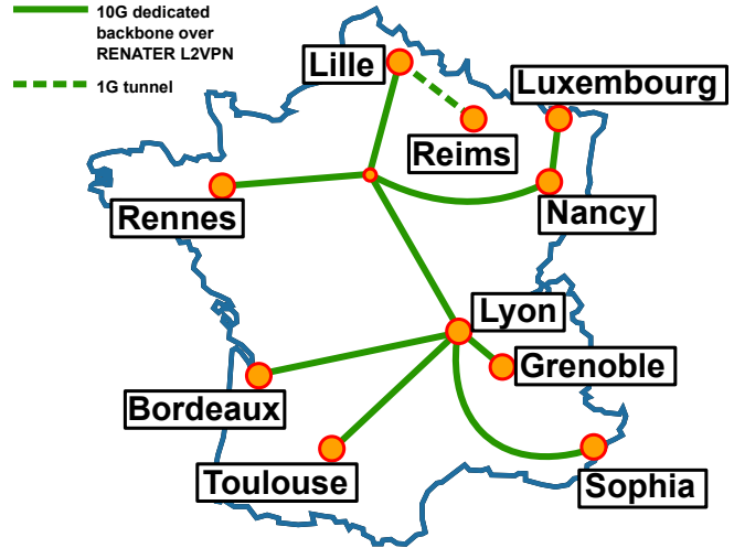
Figure 1. Grid'5000 overview
