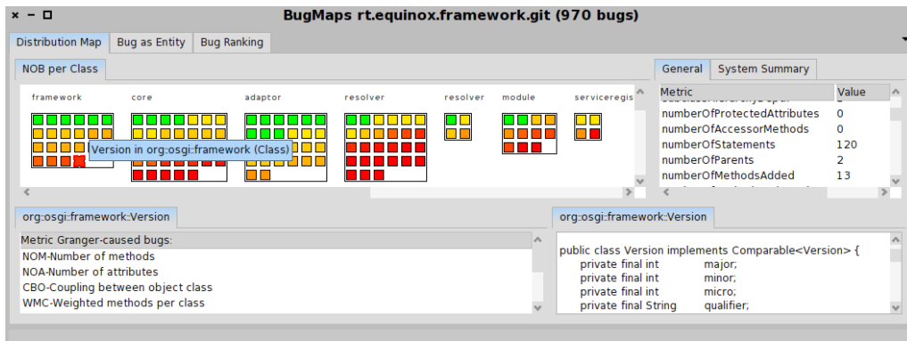
(a) Granger browser
