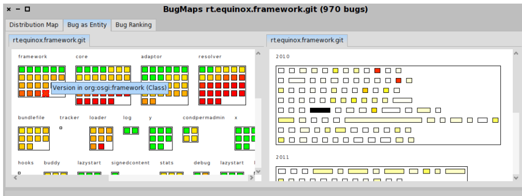
(b) Bug as Entity browser
