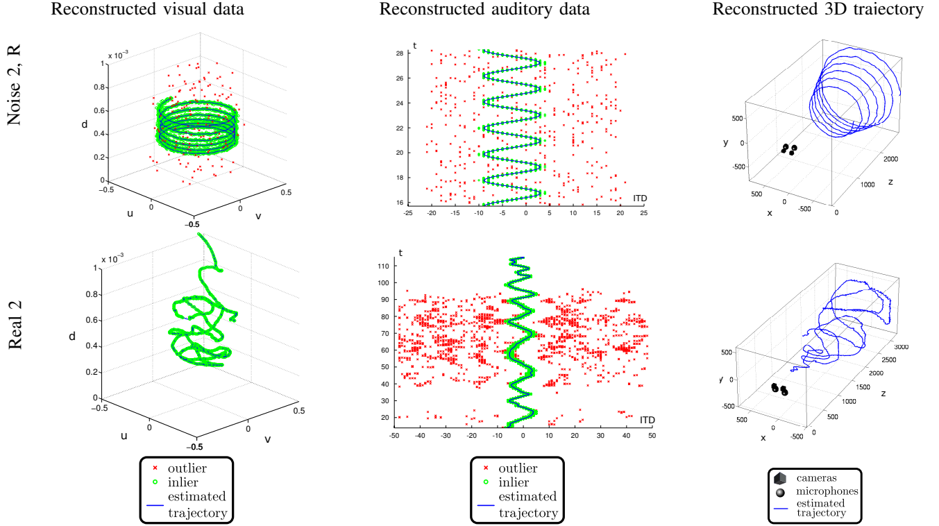
Fig. 3. Auditory and visual spaces alignment results for “Noise 2, R” simulated data experiment (top) and “Real 2” real data experiment (bottom). First two columns show results of classification of visual and auditory observations respectively into inliers ( \circ ) and outliers ( \times ). Third column shows camera and microphone locations in the 3D scene and the estimated audio-visual device trajectory. The same trajectory is shown mapped into observations spaces in the first two columns.
