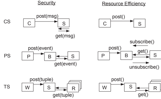
Fig. 3. Analysis of post and get \mathcal{S} and \lambda increments for success and failure.
