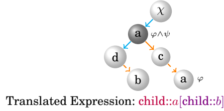
Fig. 12. Translation of Expressions and Paths.
