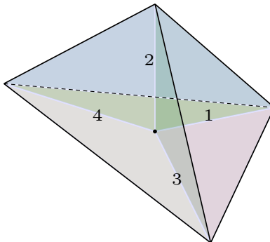
FIGURE 5. Clough–Tocher split.
