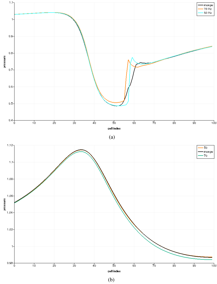
Fig. 12: Results of the Monge interpolation at 50Hz. The continuity equation and the inviscid Burgers equation are integrated starting from the initial conditions (see Fig.11). The pictures show the high-fidelity model results compared to those of the non-linear interpolation at 50Hz. (a) solution on a segment parallel to the abscissa where the pressure shows a shock wave; (b) solution on segment where the pressure is regular. These are typical results across the field.
