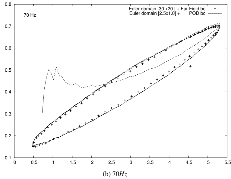
Fig. 7: CT1 case. Normal force coefficient vs. angle. Full computation vs. hybrid ROM. POD modes are build from the 50Hz simulation only.
