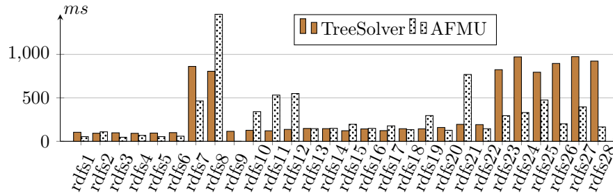
Fig. 5. Results for the UCQrdfs test suite.
