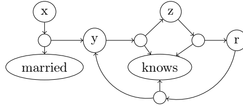
Fig. 1. Cyclic query.
