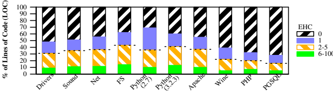
Fig. 4. Percentage of code found within functions that have 0 or more blocks of error-handling code
