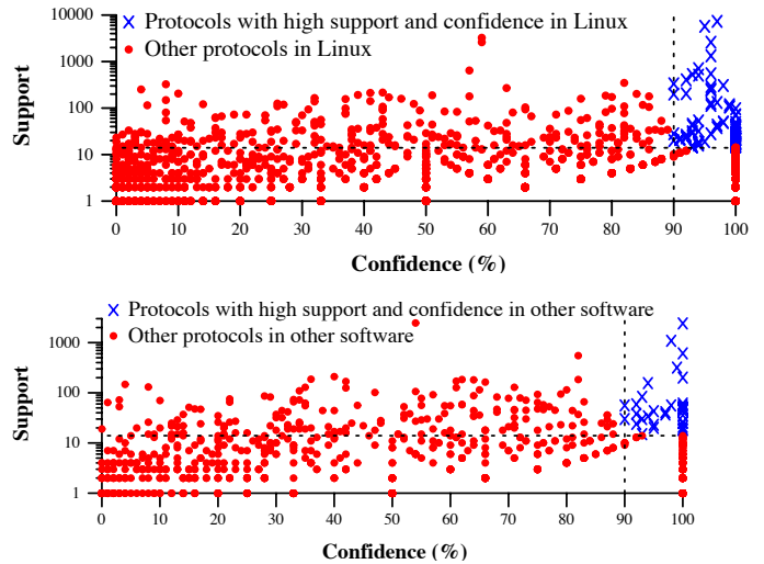
Fig. 6. Support and confidence of the identified protocols
