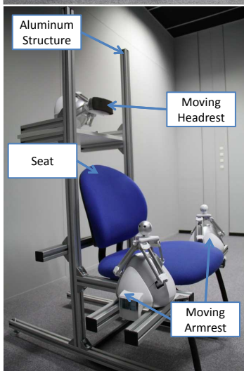
Figure 1: Prototype of the HapSeat.
