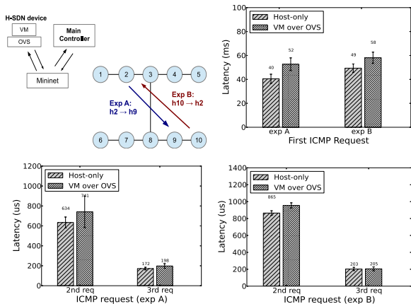
Figure 8: Impact of HSDN device.
