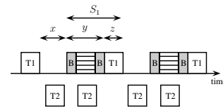
Figure 7: Relation between transmissions in neighbor nodes and backoff freezing in a non-saturated case.
