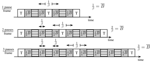
Figure 5: Illustration of the relation between \beta , \overline{np} and \overline{B} .
