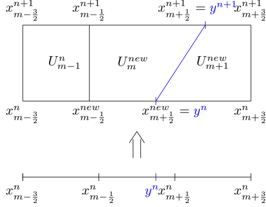
Figure 3: Local shifting of a grid point when |x_{m+\frac{1}{2}}^{n+1} - y^n| \leq \frac{h_m^n}{2} .
