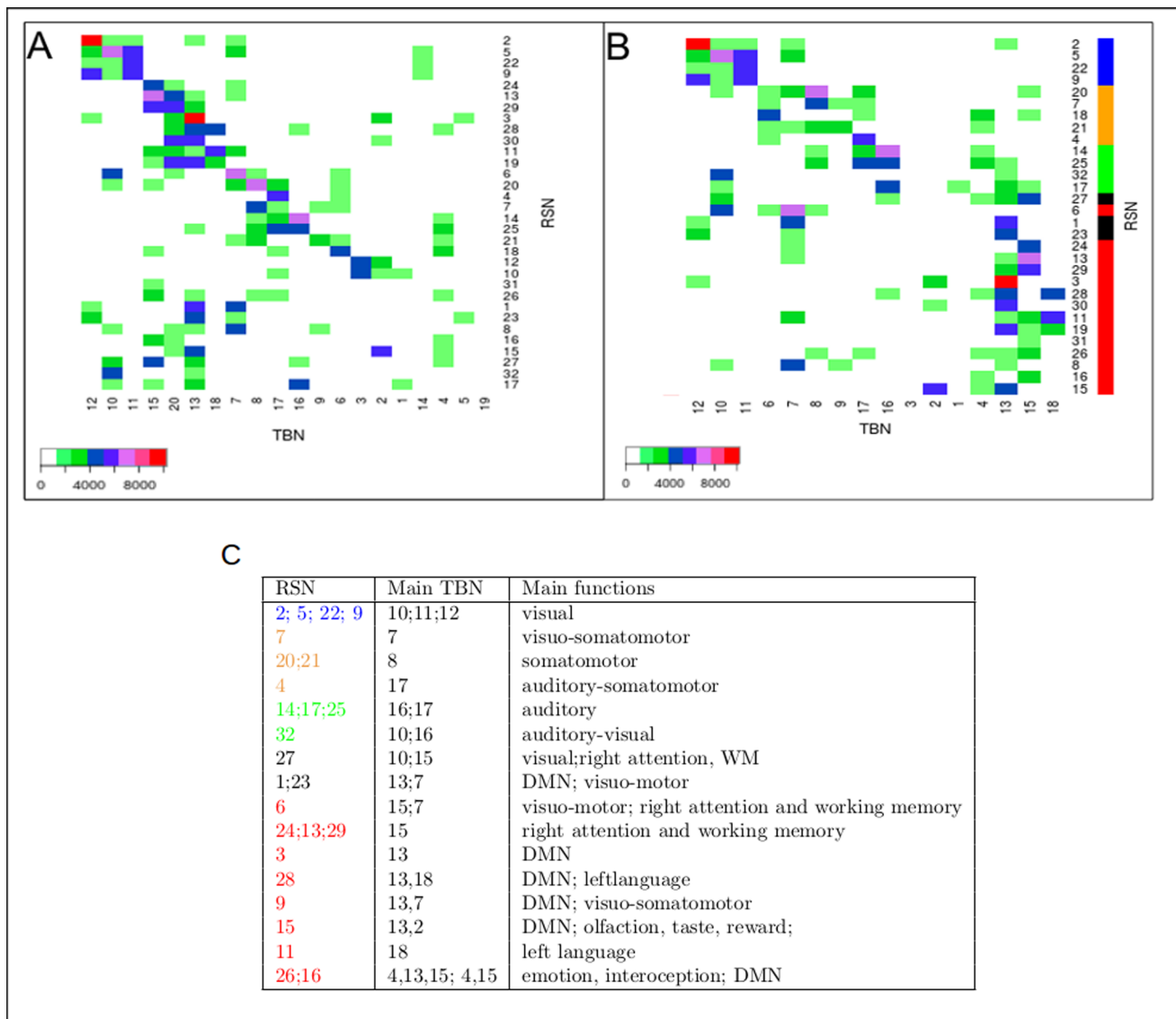
Figure 2. RSN×TBN overlap matrix. (A) RSN×TBN matrix showing overlaps (topographical similarity) between the 32 Resting State Networks (RSN, vertical axis) and the 18 reference Task Based Networks (TBNs, horizontal axis). The RSN are labeled as in Fig. 1 and the TBNs are labeled as in [14]. The RSNs and TBNs are ranked according to the maximum of their overlaps. (B) RSN×TBN matrix reorganized by applying an Expectation Maximization (EM) algorithm to display the RSN clusters having similar overlaps with the TBNs (see text for details). The RSN×TBN clusters are: C_{TBN\#1} (RSN# 2, 5, 22, 9), C_{TBN\#2} (20, 7, 18, 21), C_{TBN\#3} (4), C_{TBN\#4} (14, 25), C_{TBN\#5} (32, 17, 27) and C_{TBN\#6} (6, 1, 23, 24, 13, 29, 3, 28, 30, 11, 19, 31, 26, 8, 16, 15). The color bars (at the right of Figure 2B) indicate: visual (blue), somatomotor (orange), auditory (green), left, right and bilateral RSN (red), and RSNs of intermediate region (black). Scale bars represents the number of shared voxels. (C) This table shows the correspondence between RSNs and TBNs obtained by the maximal overlap between them, with the main sensory-motor and cognitive functions of the TBNs. The masks, labels and functions of TBNs are taken from [14]. The labels of RSNs correspond to their representativeness in the group of subjects, as in Fig. 1. The colors used for RSNs labels, are the same as color bars in Fig. 2B. doi:10.1371/journal.pone.0067444.g002
