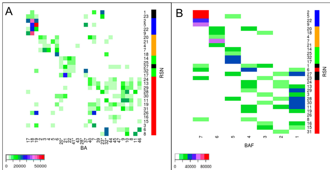
Figure 3. RSN × BA overlap matrix. (A) Matrix of 30RSN×28BA (Brodmann Area). 20*: BA20+BA38, 41*: BA41+42, 28*: BA28+BA34+BA35+BA36, 32*: BA32+BA24+BA25, 23*: BA23+BA29+BA30+BA31, (B) Matrix of 30RSN×7BAF (Brodmann Area Family), see the details concerning the BAFs and RSNs in the text. Both matrices are reorganized by applying the same Expectation Maximization (EM) algorithm as in Fig. 2C, to reveal the RSNs clusters with a similar topography on the cortical surface. The RSNs are ranked on the vertical axis according to this clustering. BA×RSN matrix clusters: C BA #1 (RSN# 1, 23, 2, 5, 22, 9), C BA #2 (20, 21), C BA #3 (4, 7, 18), C BA #4 (14, 25, 27, 32, 17), C BA #5 (24, 13, 29, 28, 30, 11, 19, 31, 26, 16), C BA #6 (3, 15) and C BA #7 (6, 8). BAF × RSN matrix clusters: C BAF #1 (RSN# 2, 22, 9, 5), C BAF #2 (4, 7, 21), C BAF #3 (18), C BAF #4 (20), C BAF #5 (25, 14, 17, 32), C BAF #6 (27, 28, 11, 29, 13, 19, 6, 26, 18, 20, 8 and 24), C BAF #7 (3, 15, 30, 16), C BAF #8 (31), C BAF #9 (23) and C BAF #10 (1). Color bars (to the right of Figures 3A, 3B) indicate: visual (red), somatomotor (orange), auditory (green), left, right and bilateral RSNs (red) and as in Table in Fig. 2C, RSNs of intermediate region are in (black). Scale bars represent the number of shared voxels. doi:10.1371/journal.pone.0067444.g003
