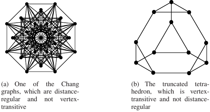
Fig. 2. Examples of graphs distinguishing the properties of distance-regularity and vertex-transitivity
