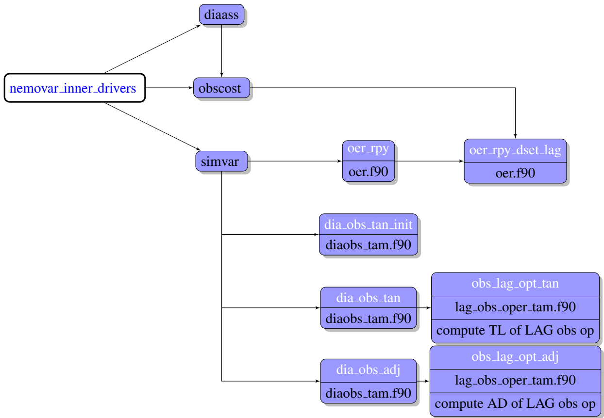
Figure 3: From the main assimilation routine, diagram of the calls ('namtst' for adjoint, gradient, tangent tests, 'namobs' for single obs.experiemment and 'namhlt' for linear tangent hypothesis)
