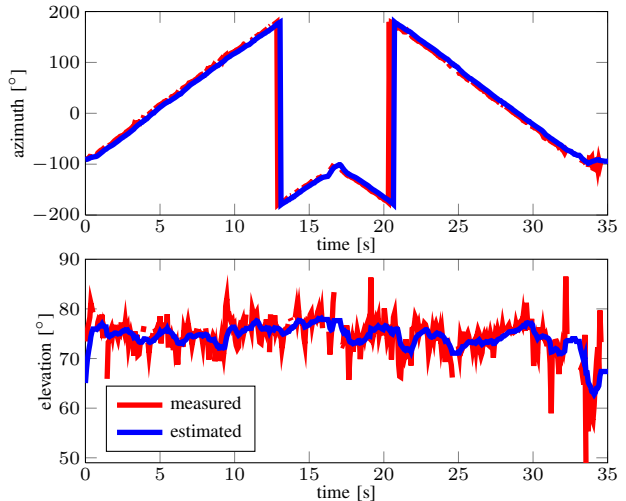
Fig. 3. Azimuth and elevation of the moving object direction
