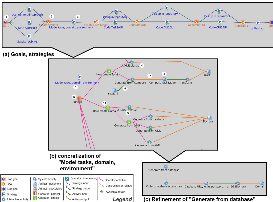
Fig.7 - UsiXML flexible process model
