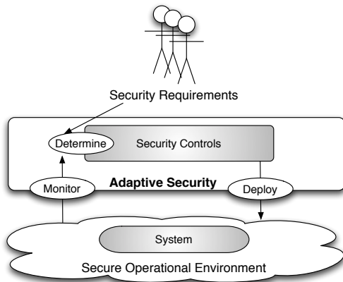
Figure 2: Adaptive Security
