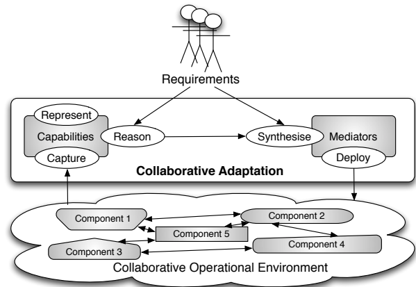
Figure 3: Collaborative Adaptation
