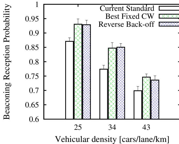
Figure 10: Beacons reception probability at 100m from the transmitter using the CW currently proposed in the IEEE 802.11p standard, the best fixed contention window and the reverse back-off mechanism under different vehicular densities.
