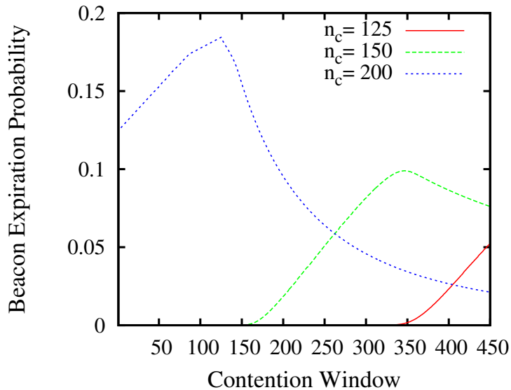
Figure 5: Beaconing expiration probability as a function of the contention window for different vehicular densities.
