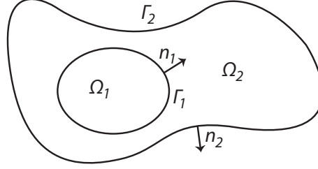
Figure 1. Cell scheme: the nucleus \Omega_1 , the cytoplasm \Omega_2 , the nuclear membrane \Gamma_1 and the cell membrane \Gamma_2 ; n_1 and n_2 are the unit normal vectors oriented outward from \Omega_1 and \Omega_2 , respectively.
