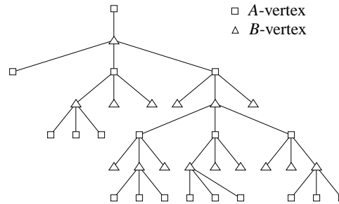
Fig. 6: A regular 4-Eulerian tree
