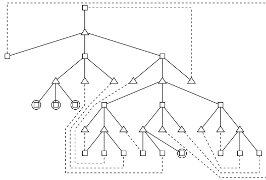
Fig. 7: Matching of an unbalanced regular 4-Eulerian tree
