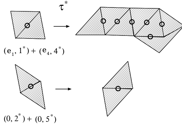
Fig. 18: The images of (e_1, 1^*) + (e_4, 4^*) and (0, 2^*) + (0, 5^*) by \tau^*
