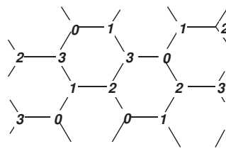
L(1,1) -labeling of G_3
