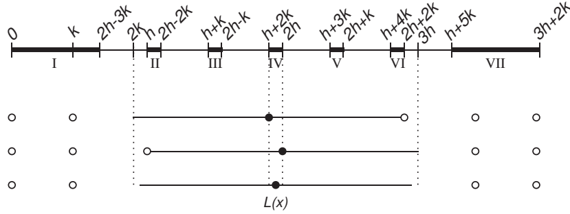
Fig. 9: The feasible intervals in the proof of Theorem 3.3.
