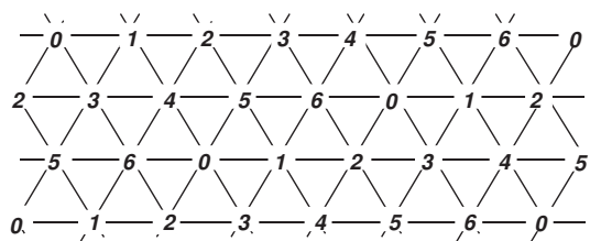
L(1,1) -labeling of G_6
