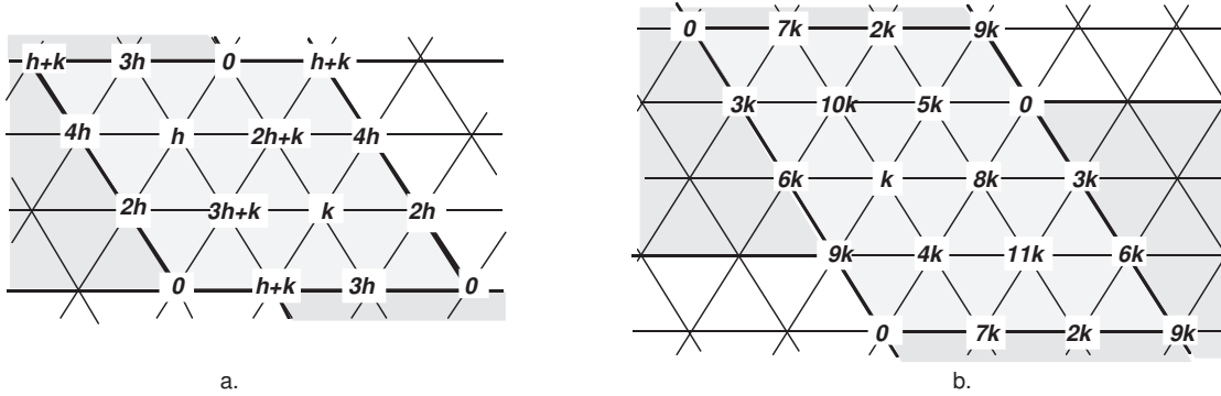
Fig. 6: Two feasible labelings of a cellular graph when 2k \leq h \leq 3k . Their span is a. 4h and b. 11k .
