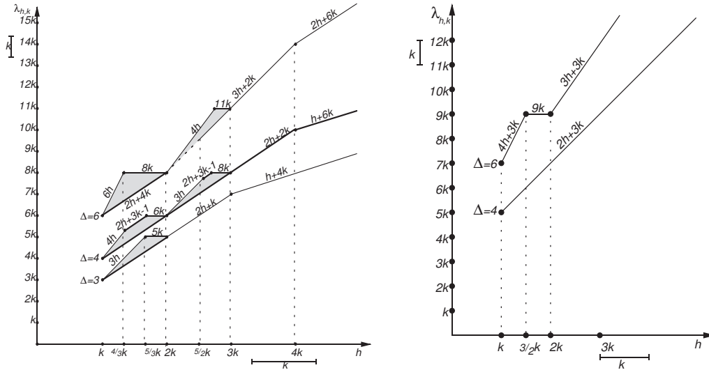
(a) Summary of the results: grey areas denote gaps between the upper and the lower bounds. Bold lines represent already known results.
