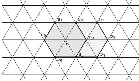
Fig. 4: A general node x and all its neighbors in a cellular graph.
