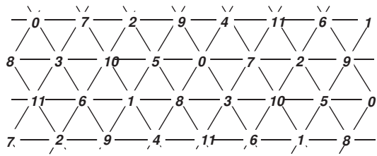
L(3,1) -labeling of G_6
