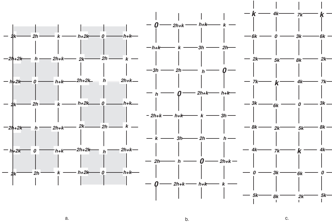
Fig. 12: a. and b. two feasible L(h, k) -labelings when when 2k \leq h \leq \frac{8}{3}k and when \frac{8}{3}k \leq h \leq 3k .
