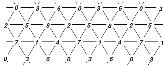
L(2,1) -labeling of G_6
