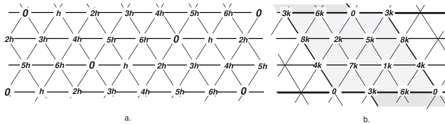
Fig. 5: Feasible labelings of a cellular graph when a. k \leq h \leq \frac{4}{3}k and when b. \frac{4}{3}k \leq h \leq 2k .
