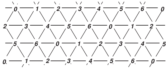
L(1,1) -labeling of G_6
