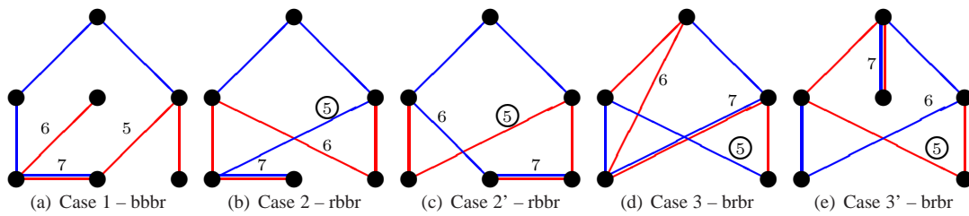
Fig. 3: Forcing a path P_5 (last three moves)
