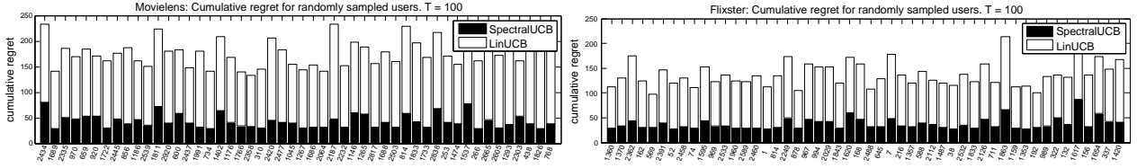
Figure 4. MovieLens and Flixster: Cumulative regret for 50 randomly chosen users. Horizontal axis shows the user number.
