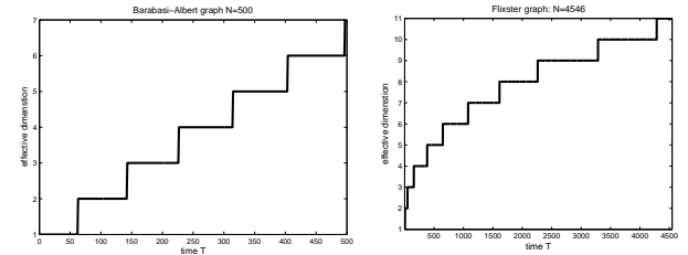
Figure 2. Effective dimension d in the regime T < N . The effective dimension for this data is much smaller than the ambient dimension D = N , which is 500 and 4546 respectively.
