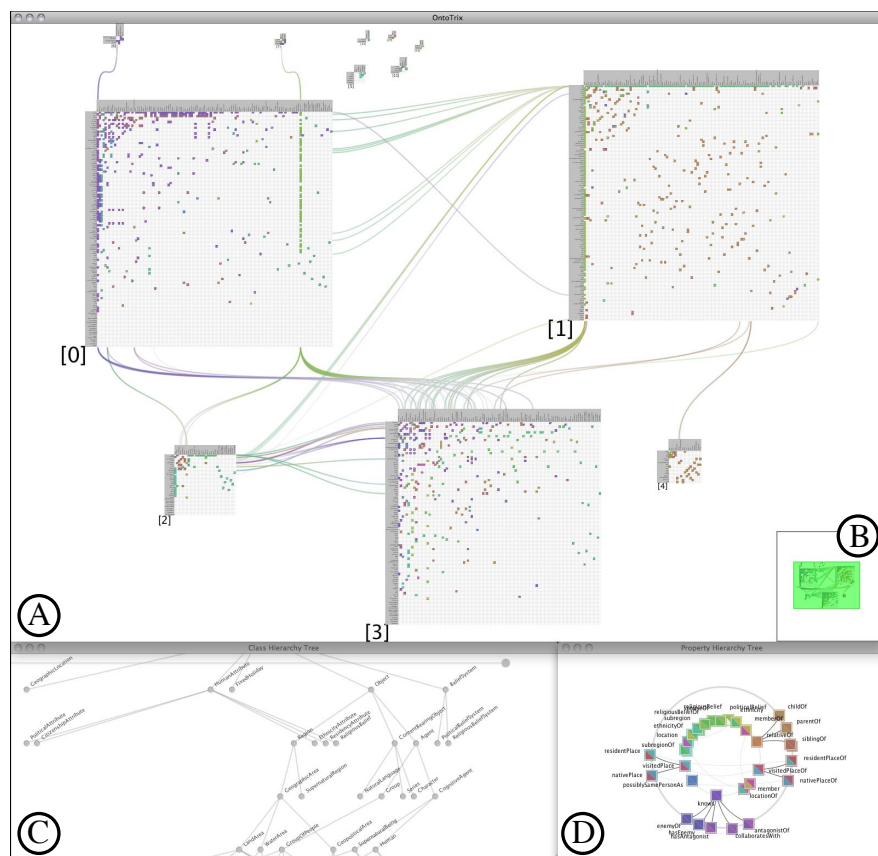
Fig. 2. OntoTrix Interface Overview: (A) Main NodeTrix view, (B) Bird's eye view, (C) Class hierarchy view, (D), Property hierarchy view.
