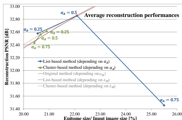
Fig. 8. Reconstructed average PSNR vs epitome size.
