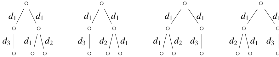
Figure 2: Drawings of \{d_1 : \{d_3 : \{\} \}, d_1 : \{d_1 : \{\} \}, d_2 : \{\} \} with different edge orders.
