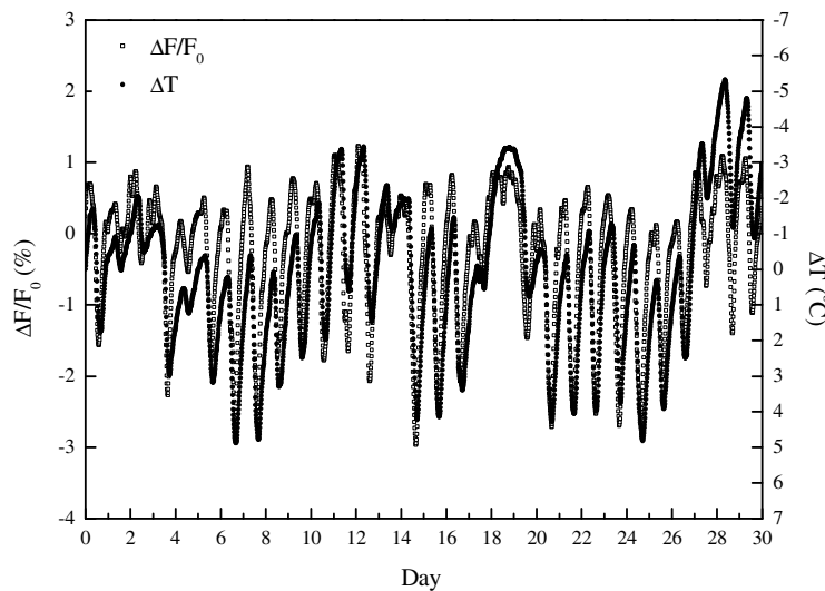
Figure 5: Time histories of denoised effective temperature and cable force
