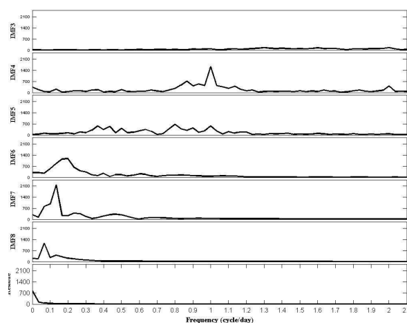
Figure 8: Fourier Spectra for IMF's of effective temperature
