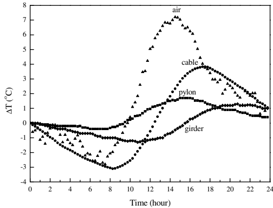
Figure 1: Daily temperature variations of air and various structural components
