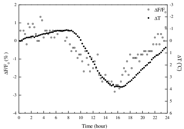
Figure 2: Daily variation of cable force and effective temperature
