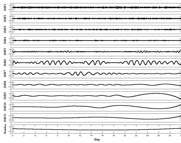
Figure 4: IMF's of the cable force from EMD
