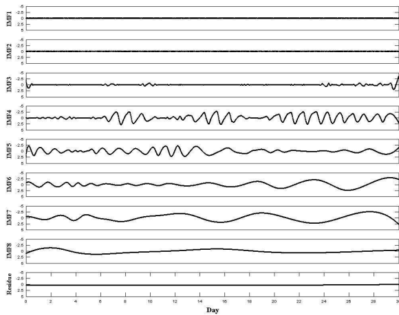
Figure 3: IMF's of the effective temperature from EMD
