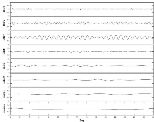
Figure 7: IMF's of the cable force from EEMD
