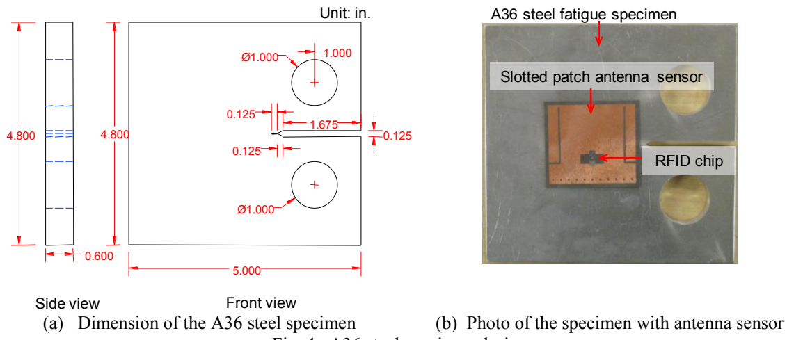
Fig. 4. A36 steel specimen design
