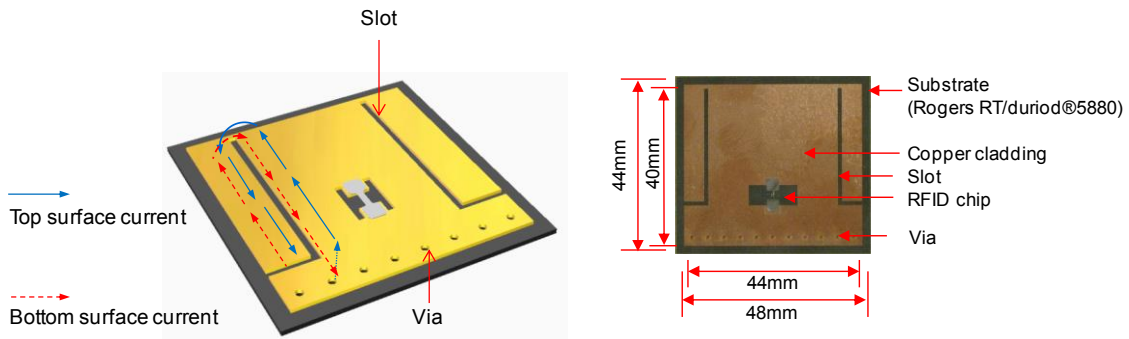
(a) Current detouring for size reduction (b) Dimension and components
