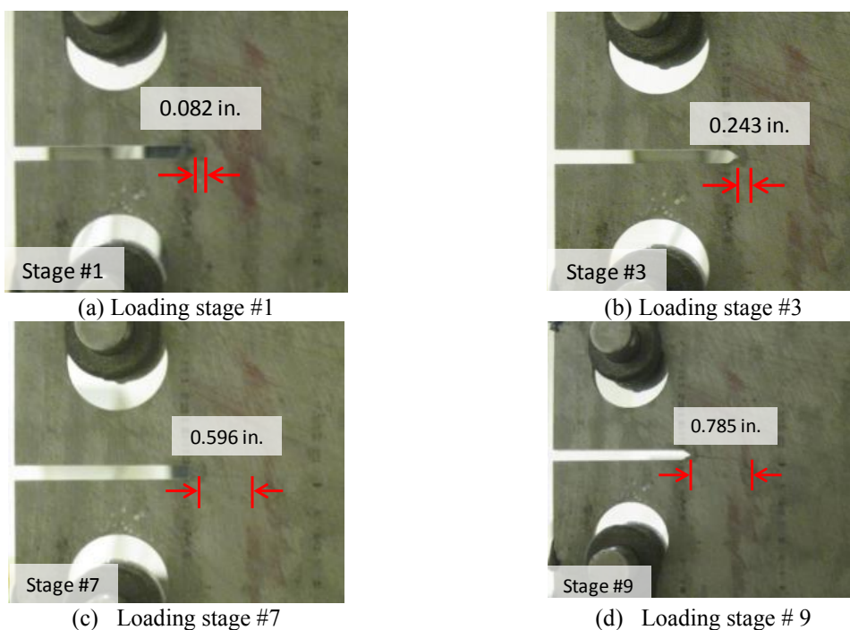
Fig. 6. Steel specimen photos at different crack length
