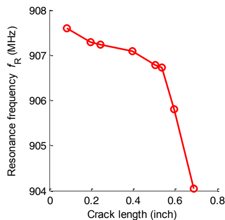
(a) Average interrogation power and threshold (b) Resonance frequency change with crack length Fig. 7. Fatigue test results of the slotted patch antenna sensor
