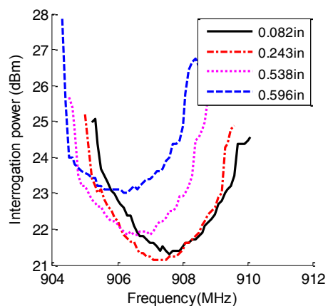
(a) Average interrogation power and threshold (b) Resonance frequency change with crack length Fig. 7. Fatigue test results of the slotted patch antenna sensor
