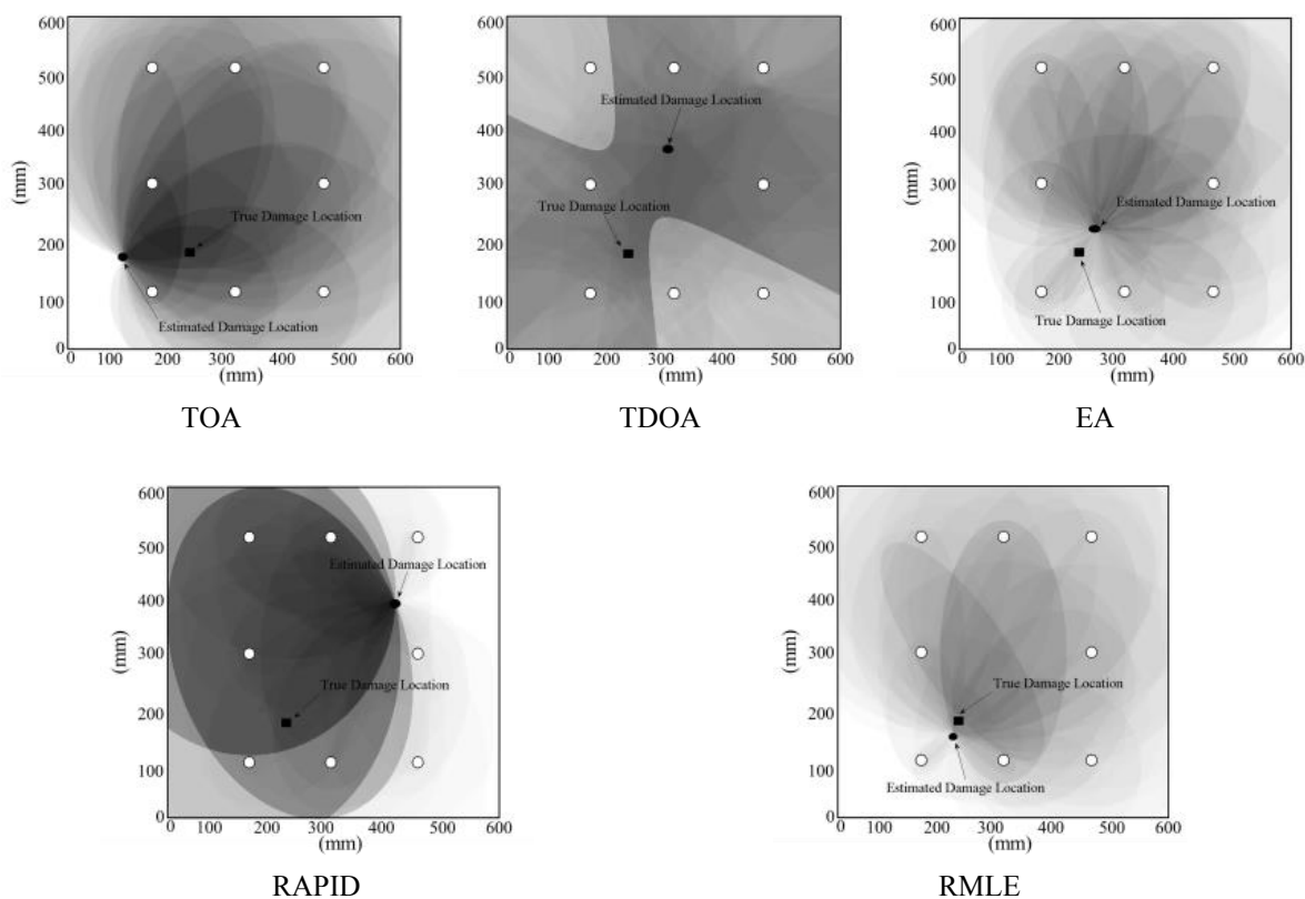
Figure 4: Application of linear methods for the damage localization.
