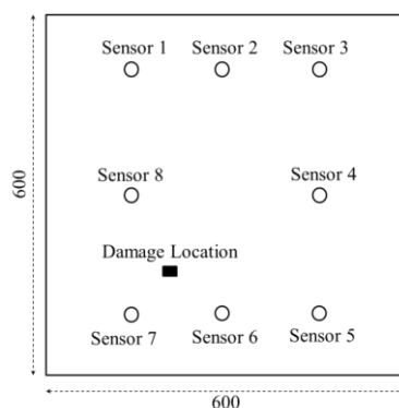
Figure 1: Sensors configuration and damage location.
