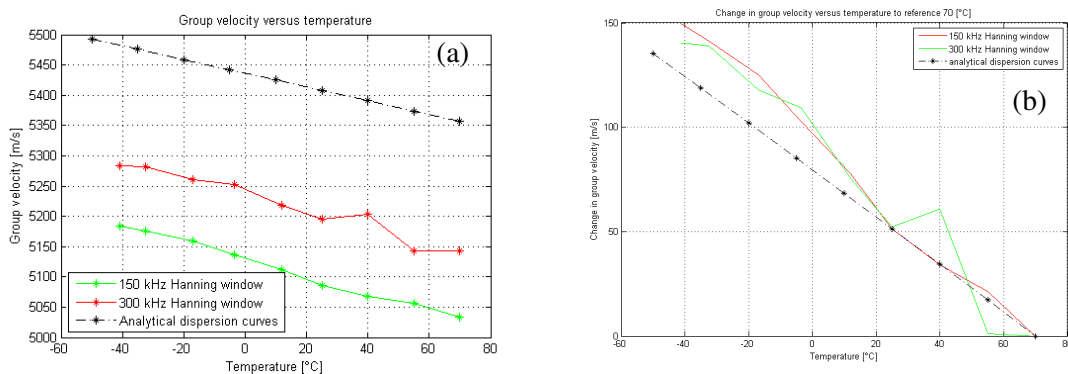
Figure 3 : The influence of temperature on wave group velocities. a) Absolute group velocity; b) change in group velocity relative to values at 70^{\circ}\text{C} .
