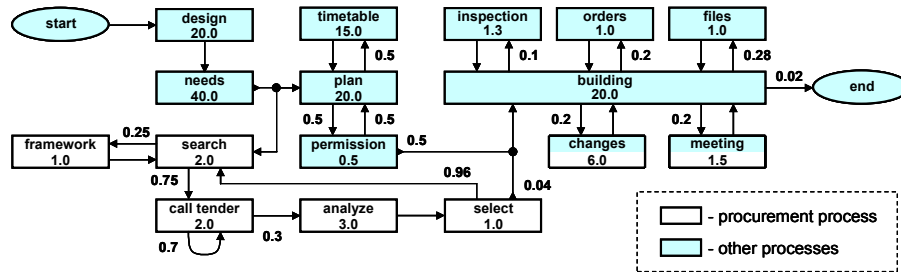
Fig. 3. Procurement Process
