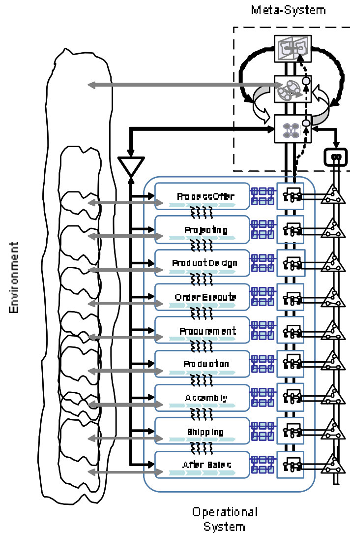
Fig. 2: Viable Production System [23] [24]
