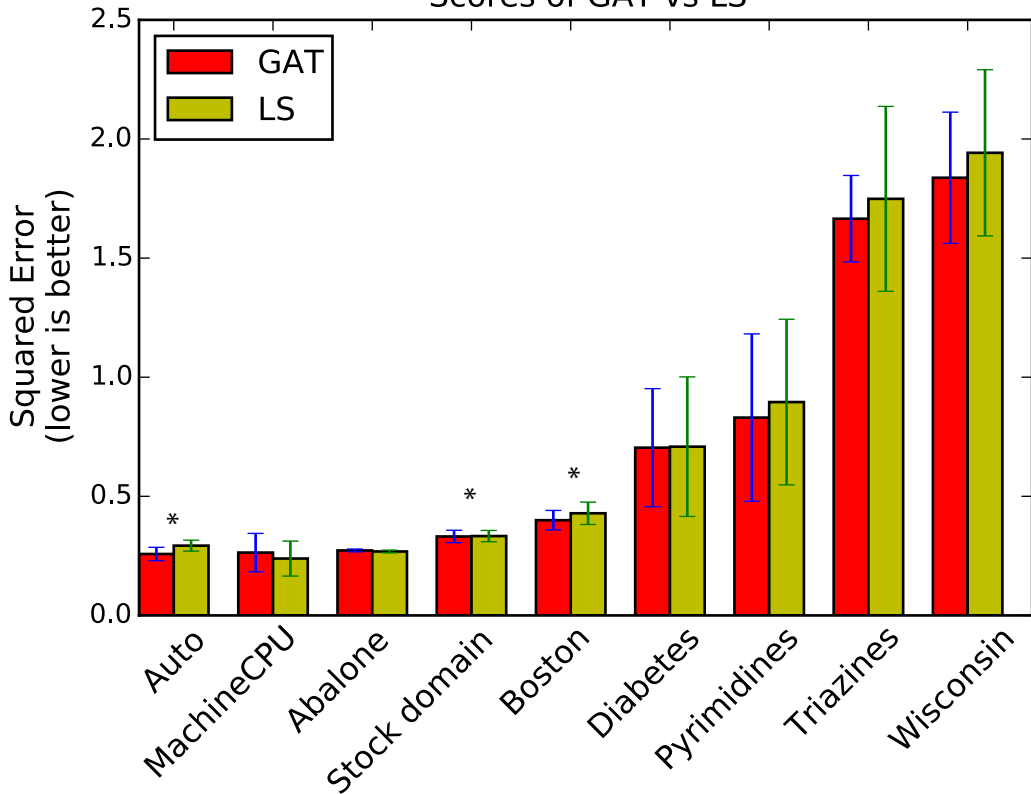
Scores of GAT vs LS
