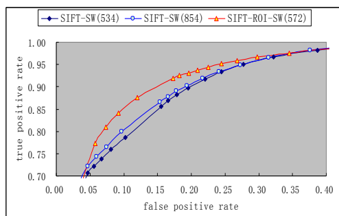
Fig. 4 The performance of BoVW based on ROI
