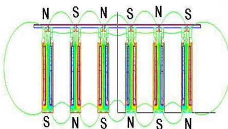
Figure 6. NS order of space distribution of magnetic field lines of magnetic force
