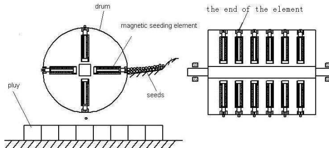
Figure1.schematic diagram of Precision Seeder
