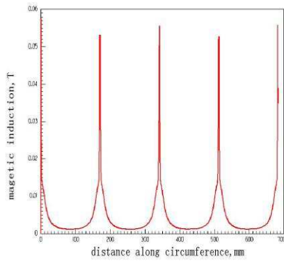
Figure 3. the curve of magnetic induction intensity in the order of NN along the circumferential direction
