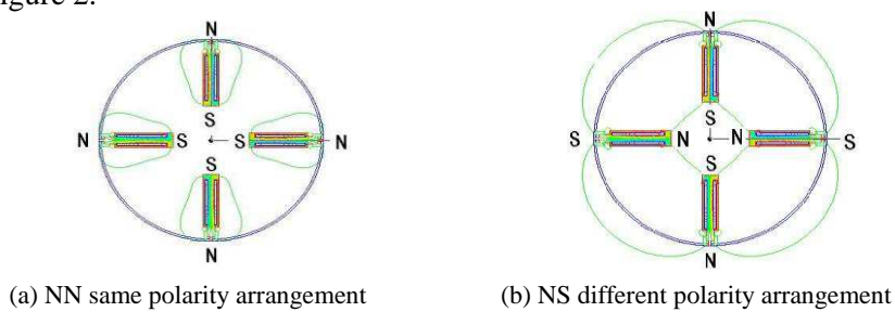
Figure 2. distributing of magnetic force line under two magnetic polar order
