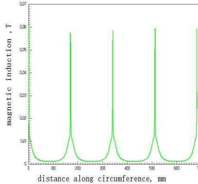
Figure 4. the curve of magnetic induction intensity in the order of NS along the circumferential direction
