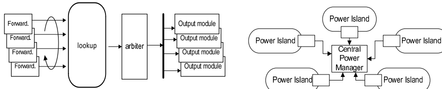
Fig. 4. Switch modules and the lookup engine
