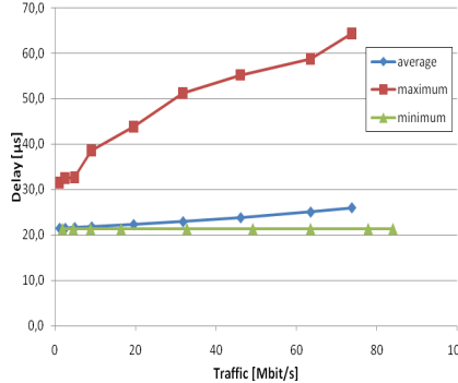
Fig. 11. Latency values for packets of 128 bytes
