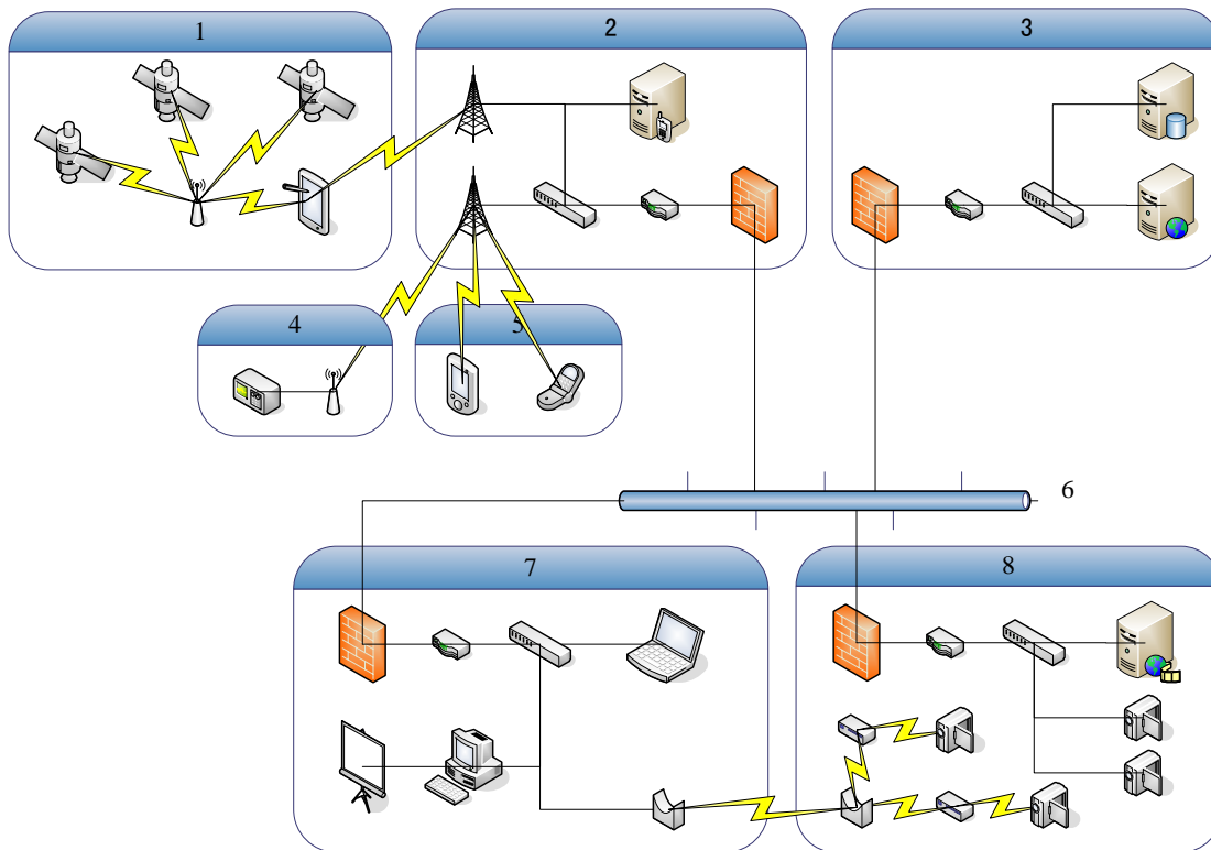
Fig.2: Network topology diagram of the network integration system of digital agriculture of Heilongjiang province①dynamic tracking system of agricultural machiney by GPS; ②telecom service provider; ③web server; ④environmental data collection; ⑤bulk SMS management; ⑥internet; ⑦unified dispatch center; ⑧remote video capture
