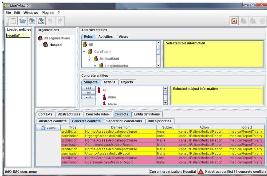
Fig. 5. Implementation of use case scenario in MotOrBAC
