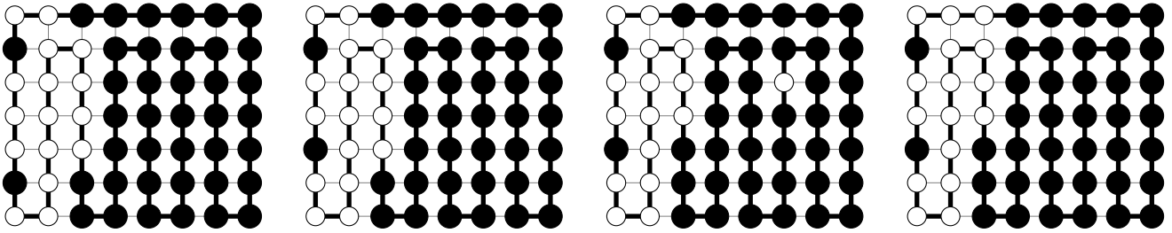
Fig. 8: Zero configurations with (N, M) = (7, 8) and k = 40 .
