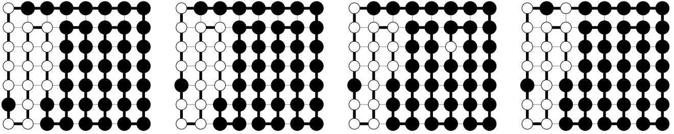
Fig. 7: One configurations with (N, M) = (7, 8) and k = 40 .
