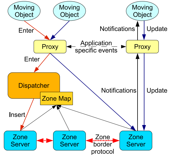
Fig. 2. Kiwano architecture
