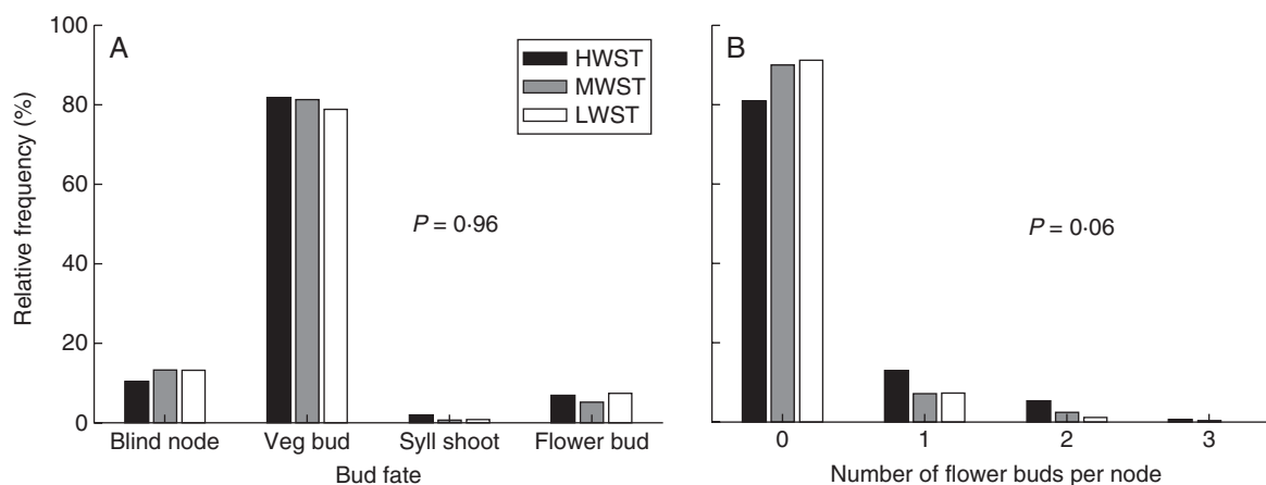
FIG. 5. Relative frequency distributions of the axillary meristem fates (A) and number of flower buds per node (B) on epicormic shoots growing in the high (HWST), medium (MWST) and low (LWST) plant water status treatments. Fisher's exact test ( P > 0.05 ) indicated no significant axillary meristem fate differences among treatments. Kruskal–Wallis ANOVA by ranks ( P > 0.05 ) indicated no significant differences in the number of flower buds per node among treatments.
