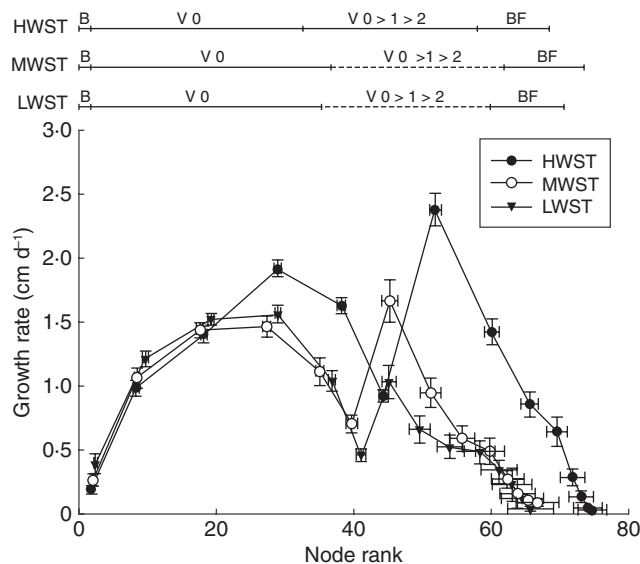
FIG. 6. Growth rate of epicormic shoots and shoot zones according to the hidden semi-Markov model for the high (HWST), medium (MWST) and low (LWST) plant water status treatments. Numbers indicate number of flower buds per node, from 0 (no flower bud) to 3 (three or more flower buds). Lines above the plot represent the mean zone lengths and dashed lines indicate zones with significantly lower zone occurrence probabilities. Letters indicate the main observation with a zone (B, blind node; V, vegetative bud; F, central flower bud).
