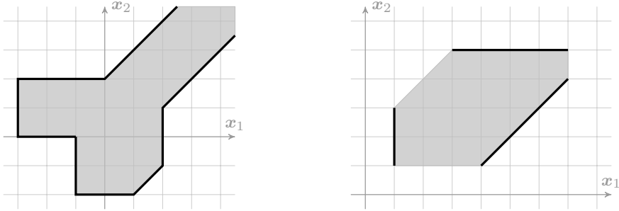
Fig. 1. Left: a tropical polyhedron (including the black border). Right: a (non-closed) zone defined by the inequalities 1 \leq x_1 < 7 , 1 < x_2 \leq 5 , -2 < x_1 - x_2 \leq 3 .
